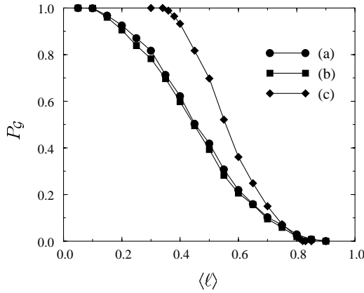
Fig. 1 – Phase diagram of the system. P_G measures the probability of having a giant component of active nodes \mathcal{G} of the order of the system size. Three different definitions of the model are represented: (a) random and dissipative, (b) random and conserved, and (c) deterministic and conserved. In all cases the size of the system has been set to N = 10^4 nodes ( 3 \times 10^4 links).
