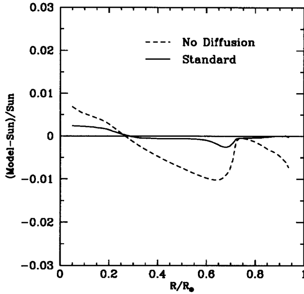
Figure 2. Comparison of sound speeds predicted by different standard solar models with the sound speeds measured by helioseismology. There are no free parameters in the models. The figure shows the fractional difference, \delta c/c , between the predicted model sound speed and the measured [24,25] solar values as a function of radial position in the sun ( R_{\odot} is the solar radius). The dashed line refers to a model [17] in which diffusion is neglected and the dark line represents a model [17] which includes diffusion and recent improvements in the OPAL equation of state and opacities [26,27]. This figure is adapted from [18].
