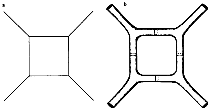
STRING THEORY'S SMOOTHING EFFECT is apparent when one compares a Feynman graph (a) with its stringy counterpart (b). The string diagram has no singular interaction points. FIGURE 7
