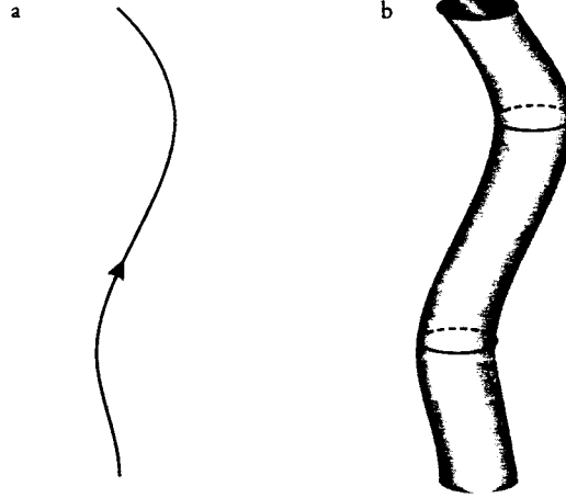
PARTICLES AND STRINGS. a: A point particle traces out a one-dimensional world-line in spacetime. b: The orbit of a closed string is a two-dimensional tube, or “world-sheet,” in spacetime. FIGURE 6
