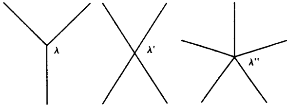
ARBITRARY FACTORS are associated with arbitrary branchings of particles in conventional field theory. In the Standard Model of particle physics, this freedom leads to about 17 parameters whose values are not understood theoretically. FIGURE 5
