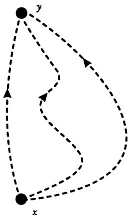
SEVERAL FEYNMAN DIAGRAMS contributing to the same physical process. FIGURE 4
