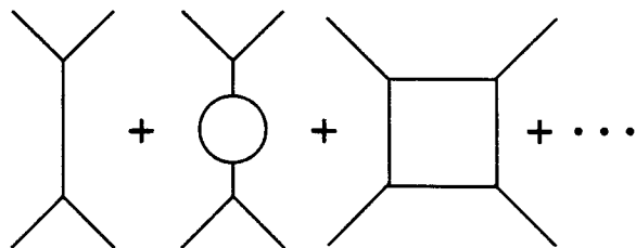
SEVERAL FEYNMAN DIAGRAMS contributing to the same physical process. FIGURE 4
