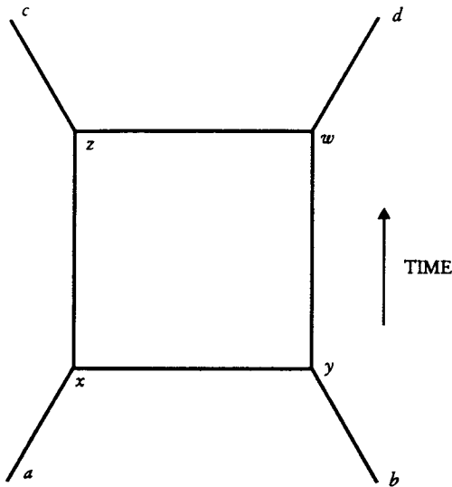
A FEYNMAN DIAGRAM with two incident particles at spacetime events a and b , and two outgoing particles at c and d . Time flows vertically. The particles interact by branching and rejoining at the spacetime events x , y , z and w . Those vertices lead to fundamental problems in field theory. FIGURE 2
