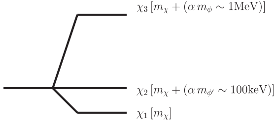
FIG. 4. Spectrum of exciting dark matter.
