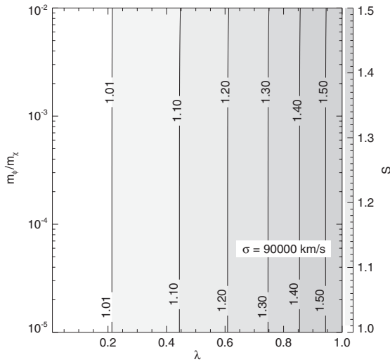
FIG. 3. Contours for the Sommerfeld enhancement factor S as a function of the mass ratio m_\phi/m_\chi and the coupling constant \lambda , at a temperature T_{\text{CMB}} = m_\chi/20 (the enhancement is integrated over a Boltzmann distribution with \sigma = 0.3c ).
