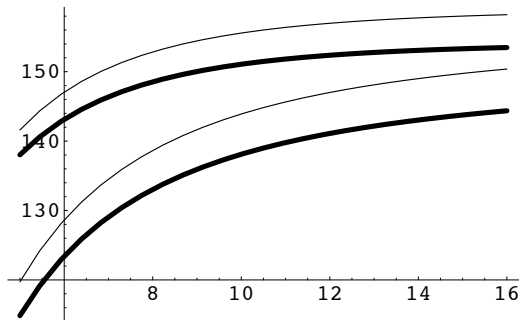
Figure 5: The Higgs mass in GeV, as a function of \log_{10}(m_S/\text{GeV}) . The thick line is for m_t = 174 GeV, the thin line for m_t = 178 GeV, while lower lines are for \cos 2\beta = 0 and the upper lines for \cos 2\beta = 1 .
